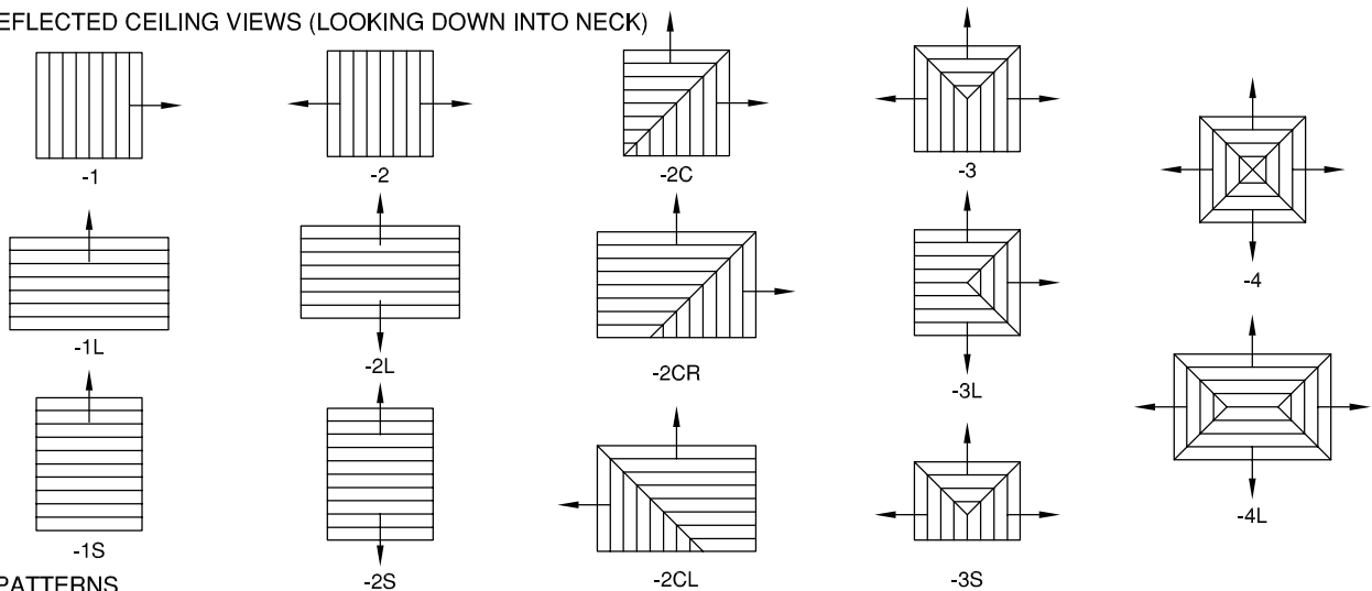
DIFFUSER PATTERNS
